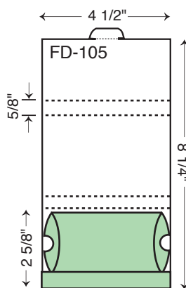
Dieline layout
